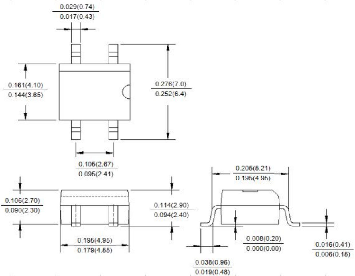
elevation view
